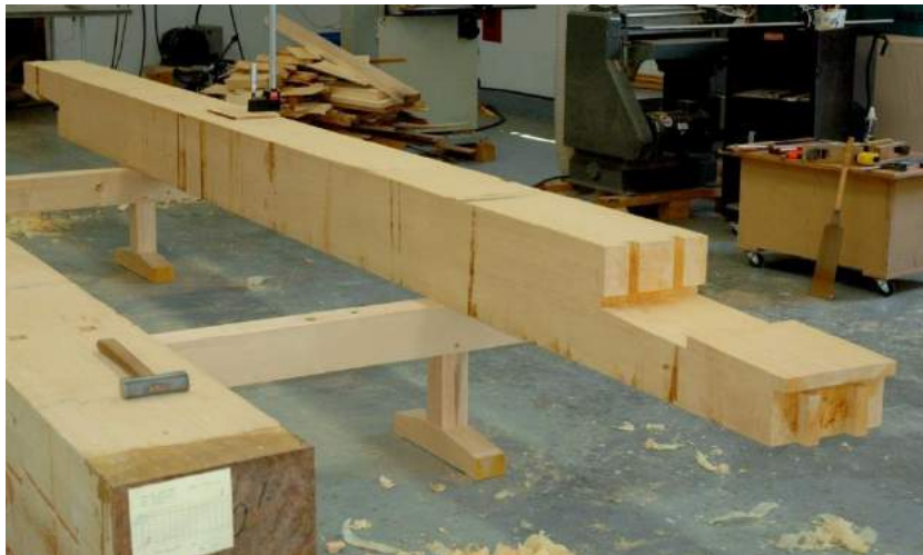
Japanese Kanawa Tsugi scarf joint; photo credit – Torij, Inc.
